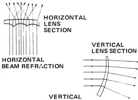
Fig. 91 Headlight Beam Refraction
