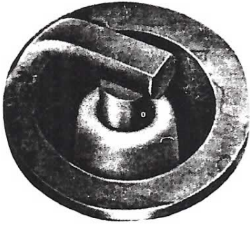
Fig. 70 Normal Spark Plug Firing Tip
