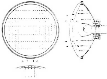
Fig. 90 Headlight Beam Reflection and Refraction
